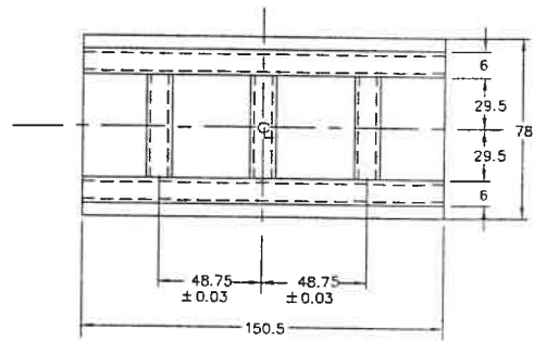
BASE DETAIL BOTTOM VIEW
